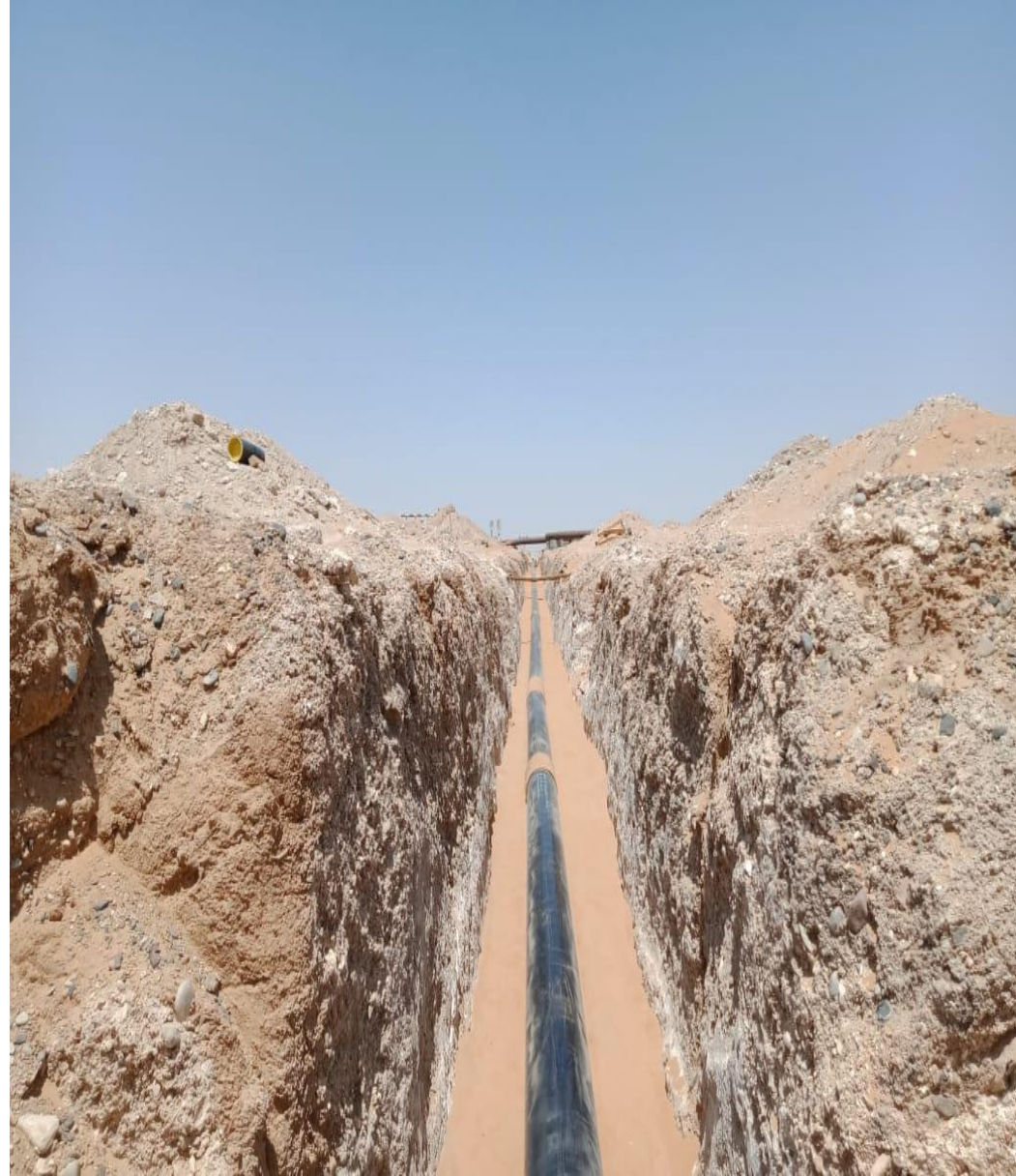
TRENCH EXCAVATION & PIPE LAYING
